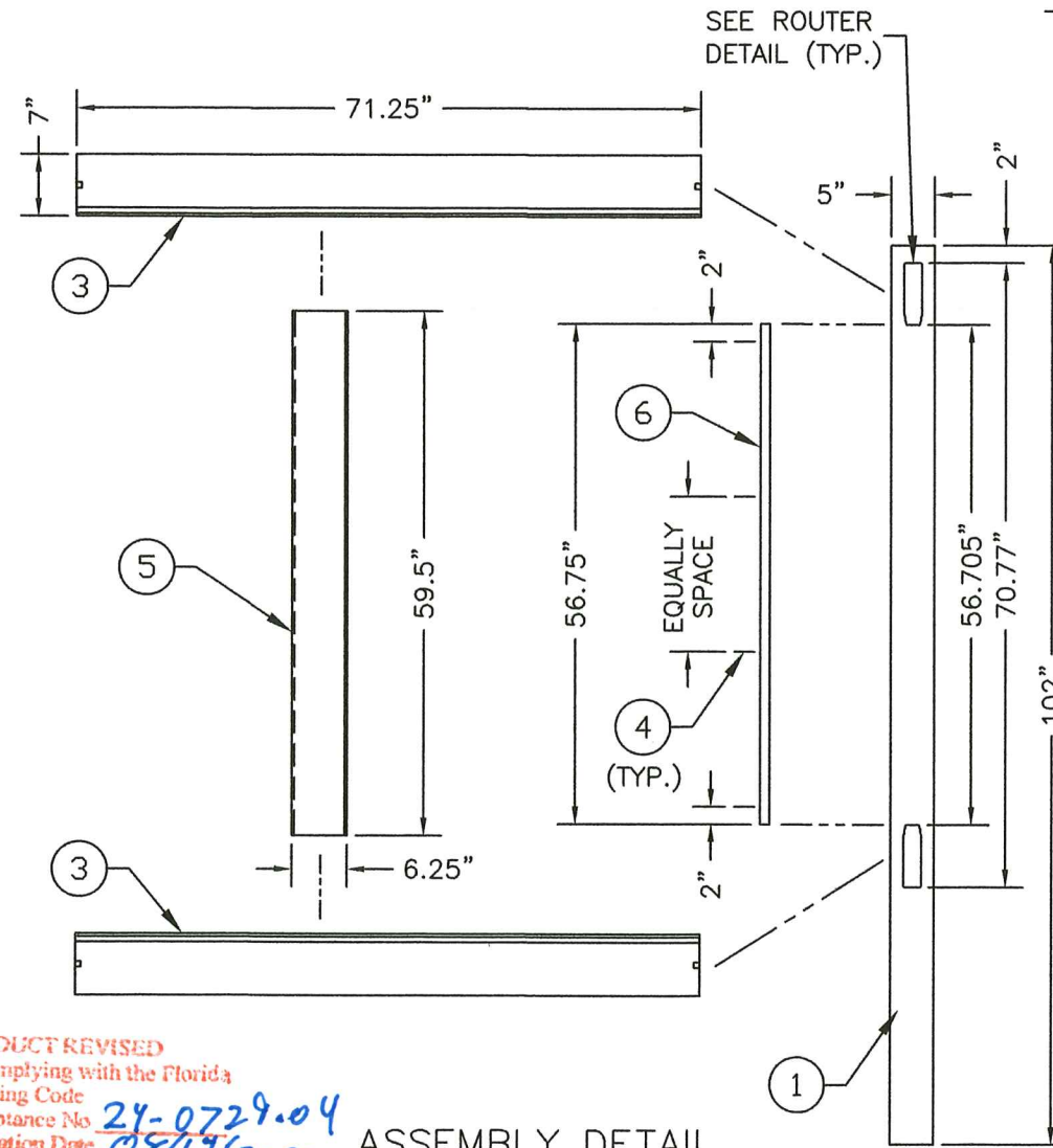
ASSEMBLY DETAIL
