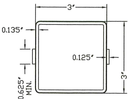
③ 3" X 3" RAIL
