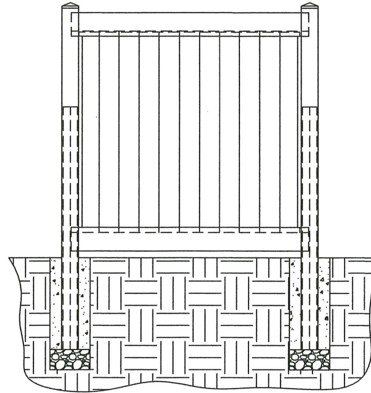
TAHOE II FENCE
