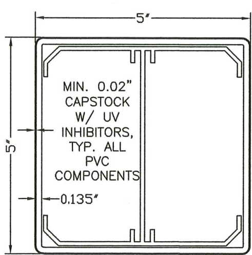
① 5" X 5" POST
